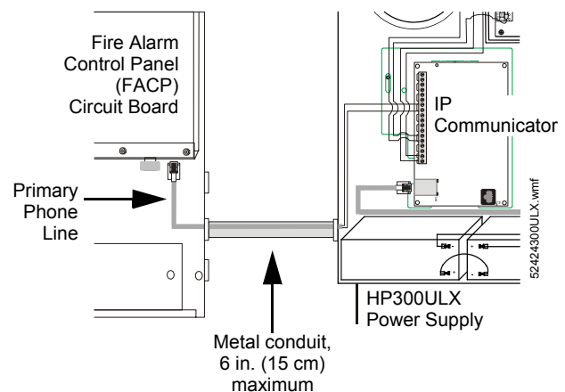
Mounting in the HP300ULX Power Supply
